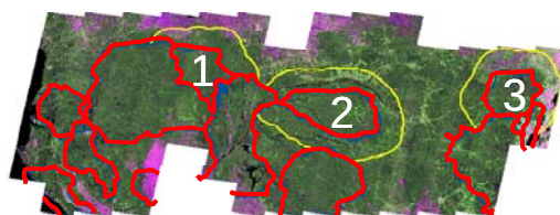
Figure 3. Annual deforestation rates were calculated for selected CARPE 2 landscapes (red) and a 100-km buffer around these landscapes (yellow). The landscapes investigated are 1) Sangha Tri-National, 2) Maringa-Lopori-Wamba, and 3) Ituri-Epulu-Aru.
