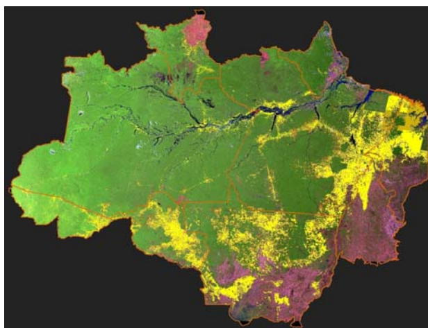
Figure 5. Deforestation in the Brazilian Amazon.
