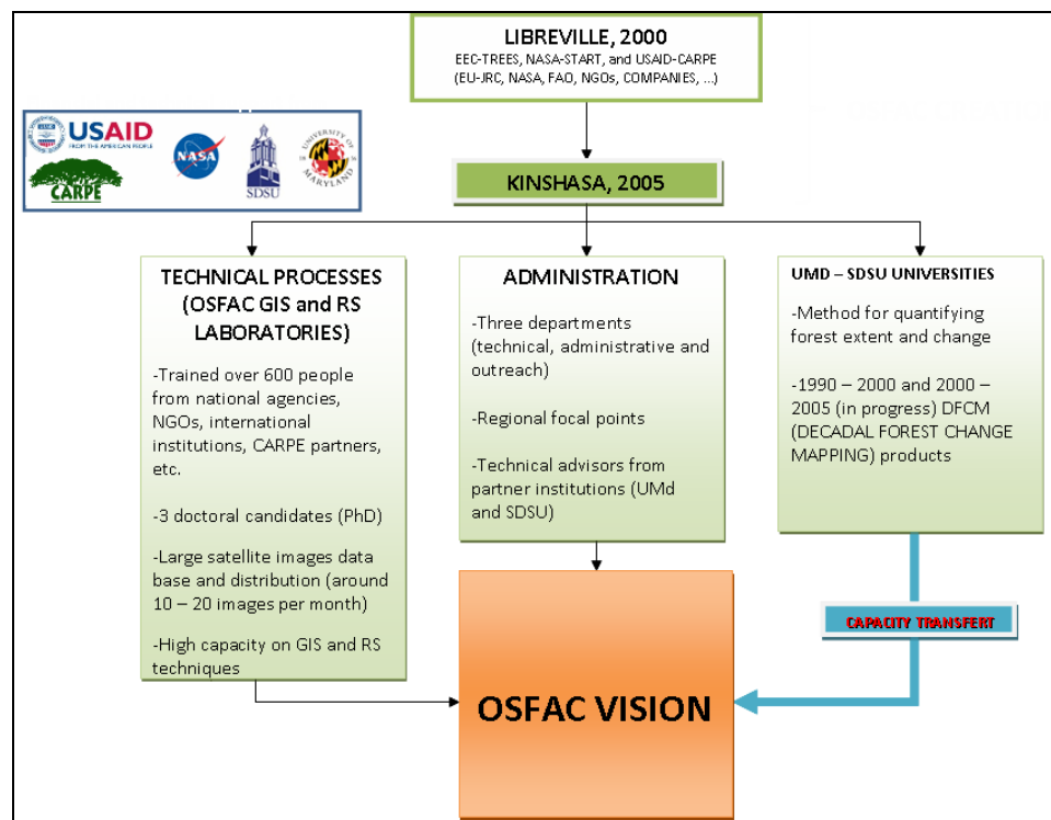
Figure 1. OSFAC overview.
