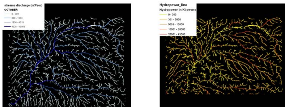
Figure 5. October Stream discharge and gross hydropower potential.
